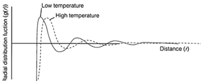
Fig. 1. Radial distribution function for an idealized liquid.
