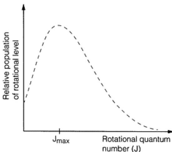
Fig. 2. Relative population of the rotational energy levels of a linear molecule as function of rotational quantum number J .
