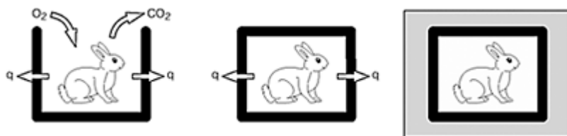
Fig. 1. Examples of an open system (left), a closed system (center) and an isolated system (right).
