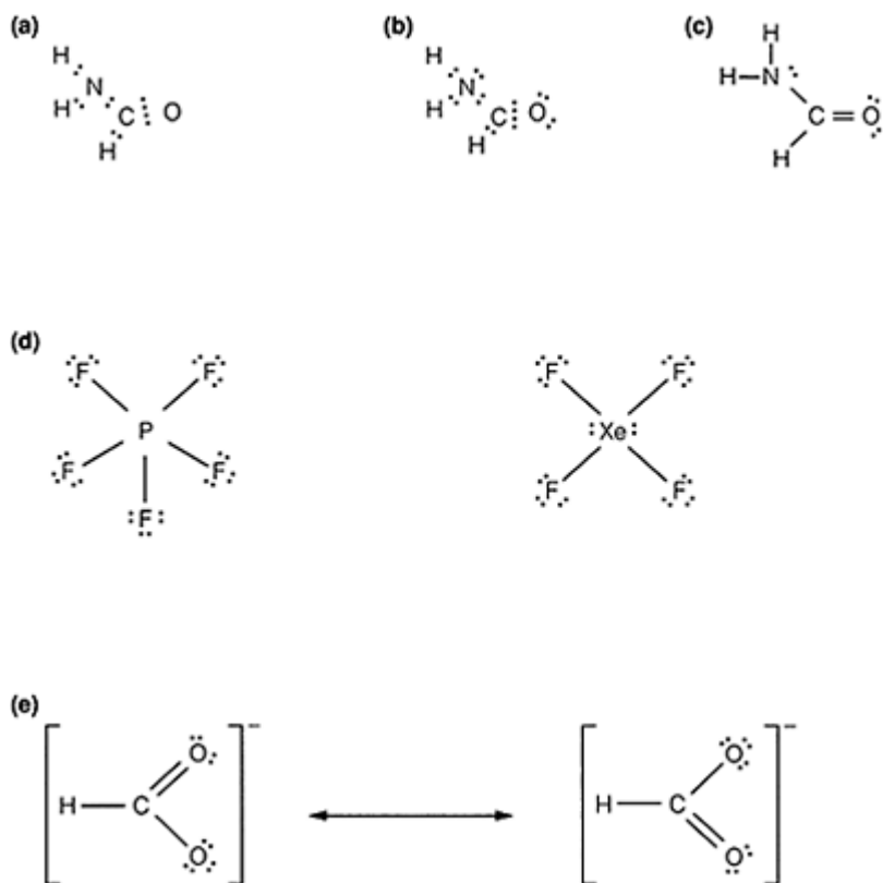
Fig. 1. (a)–(c) Development of a Lewis bonding scheme for \text{HCONH}_2 . Examples of (d) hyper-valency, and (e) resonance hybridization.
