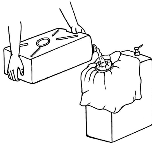
Method S
