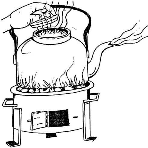
Method T
